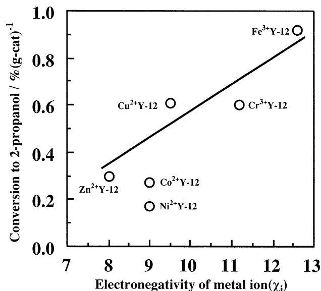
Fig. 4. Correlation between catalytic activities of metal ion-exchanged zeolites and the electronegativities of metal ions (χ i ). χ i reported by Tanaka et al. (Ref. 12) was used. Reaction conditions were the same as those in Table 2.
